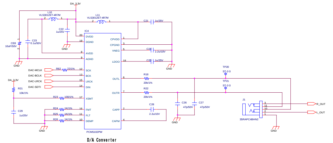
D/A Converter
